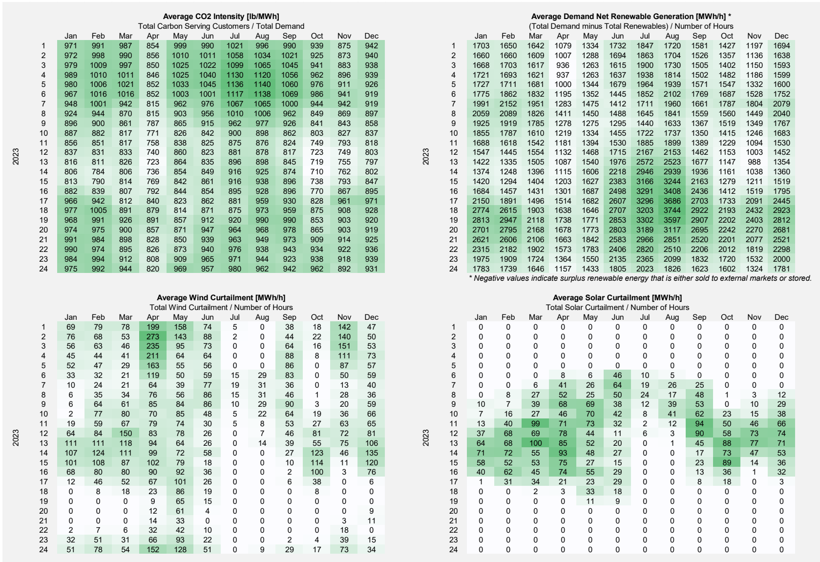
Figure R1 – 2023 Heat Maps of the Modeled Preferred Portfolio: Average CO2 Emissions, Demand Net of Renewables, Curtailment of Wind, and Curtailment of Solar
